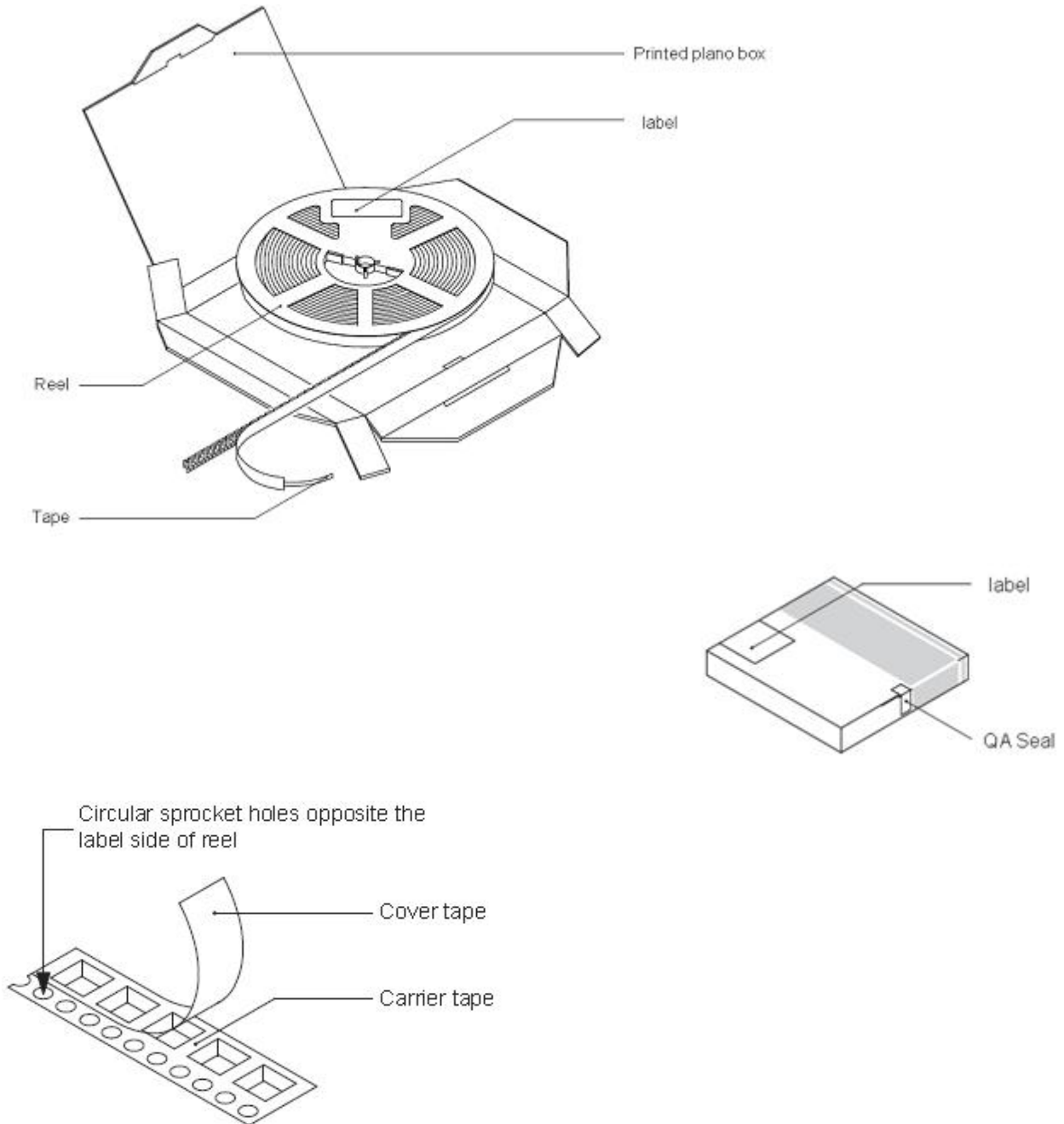
Fig.1- Reel pack for 0201 Flipship
